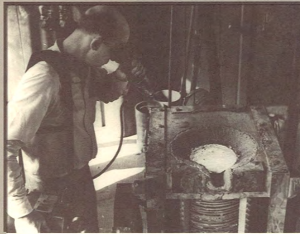
This optical pyrometer (ca. 1954) enabled a production engineering researcher to measure temperature in this induction furnace. The device utilized the human eye to compare a heating element to visible, radiating color. Before the advances in electronic imaging technology of the 1980s, many devices tried to assist natural vision in making measurable observations.
