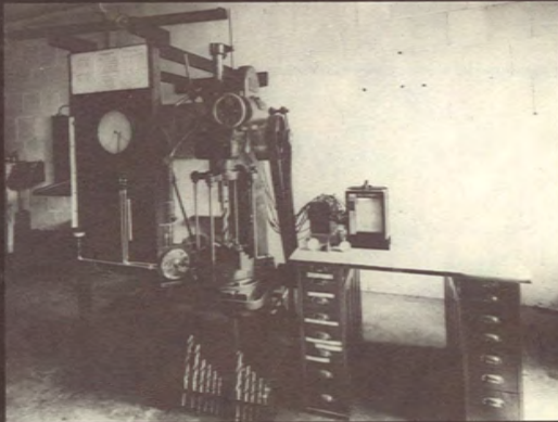
This drilling dynamometer set-up (left) and lathe set-up for tool life tests (right) were designed and built by O.W. Boston (ca. 1923-30) in "The Shops."
