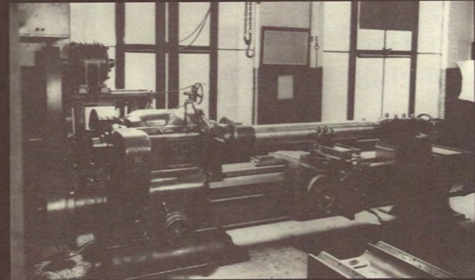
This drilling dynamometer set-up (left) and lathe set-up for tool life tests (right) were designed and built by O.W. Boston (ca. 1923-30) in "The Shops."
